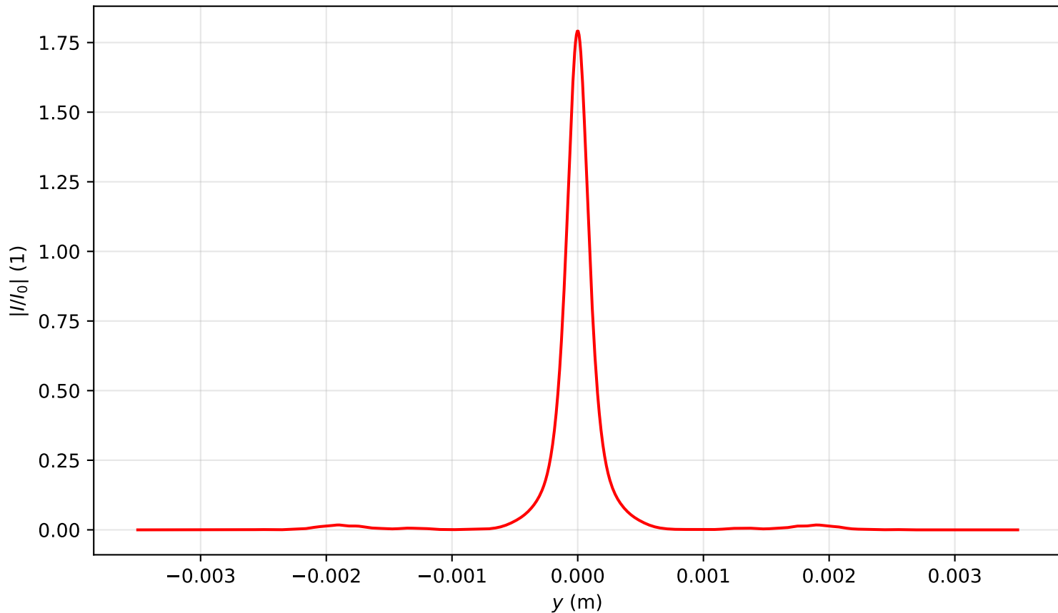
Intensity profile I(x=0, y, z=1.115)/I_0 , P_{in}=5.0P_{cr} , artificial time
